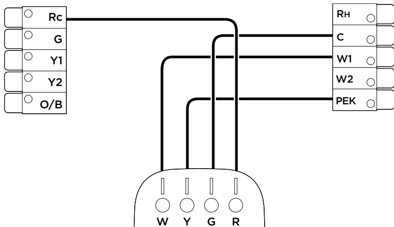
Power Extender Kit (at your HVAC system)
